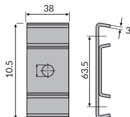
Double clamp Part: MV-329 Code: 32901
