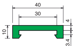
Flat clip on profile
