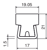
19.05mm T guide rail Part: MV-143 Code: 14301C-3m
