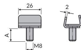
Single clamp M8 Part: MV-330 Code: 33001 a=15 Code: 33002 a=26 Code: 33003 a=20
