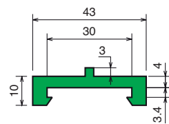
Flat clip on profile with nose
