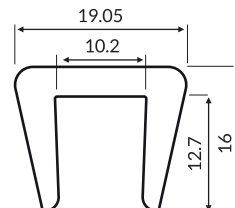
10mm snap on Part: MV-1011 Code: 101103-30m
