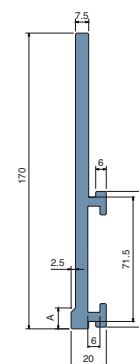
170mm side guide Part: MV-187 Code: 18730BC-3m
