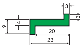
Z profile reinforced
