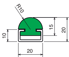
Standard guide rail Part: MV-134 Code: 13401C-3m
