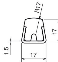
Modified guide rail Part: MV-120 Code: 12001C-3m
