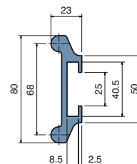
80mm side guide Part: MV-183 Code: 18301BC-3m
