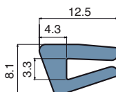
Neck guide to fit 3mm
