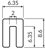
1.5mm snap on Part: MV-1000 Code: 100003-30m
