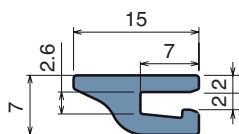
15mm neck guide
