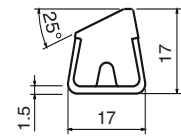
25° guide rail Part: MV-152 Code: 15201C-3m
