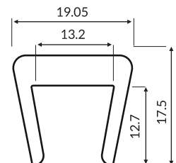
12mm/13mm snap on Part: MV-1012 Code: 101203-30m
