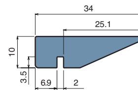
34mm neck guide
