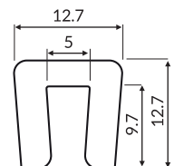
5mm snap on Part: MV-1006 Code: 100603-30m
