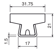
31.75mm T guide rail Part: MV-123 Code: 12301C-3m
