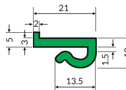
Z-clip profile with nose
