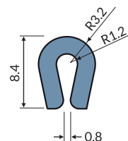
Neck guide to fit 1.8-2mm
