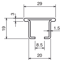
Stainless steel profile
