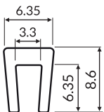
3mm snap on Part: MV-1002 Code: 16603-30m
