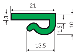
Z-clip profile without nose
