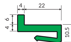
Z-clip profile with nose
