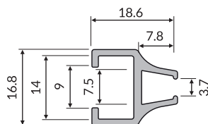
Aluminium rail bottle guide
