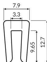
3mm snap on Part: MV-1004 Code: 100403-30m
