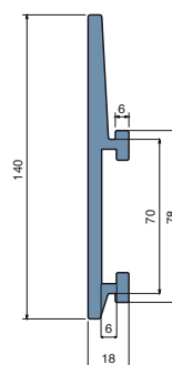
140mm side guide Part: MV-193 Code: 19320BC-3m
