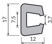
Aluminium rail bottle guide
