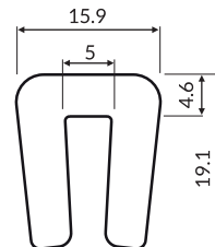
4mm/5mm snap on Part: MV-153 Code: 15303-30m
